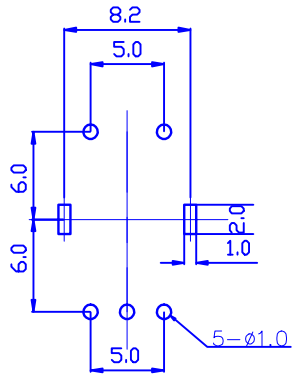
PCB.MOUNTING.HOLE.DETAIL
